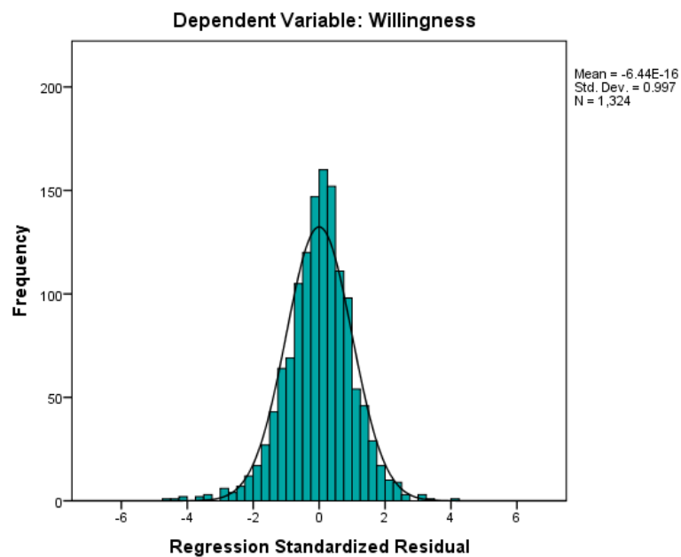
Figure 11. Frequency Distribution Histogram of Residuals
